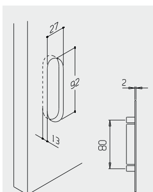
FRESATURA PER NICCHIA MILLING FOR FLUSH HANDLE
