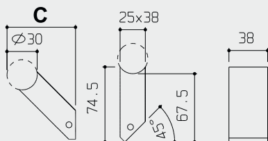
SUPPORTI INCLINATI SLANTED SUPPORTS
